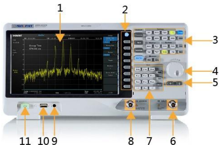
Figure 1-6 The Front Panel
