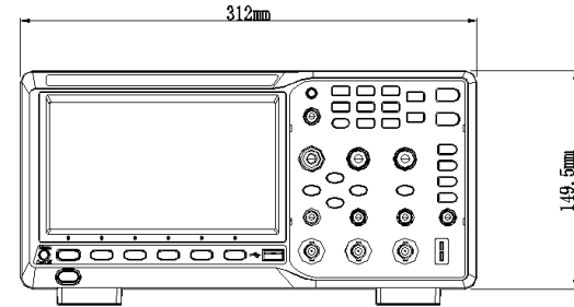
Figure 1 Front View
